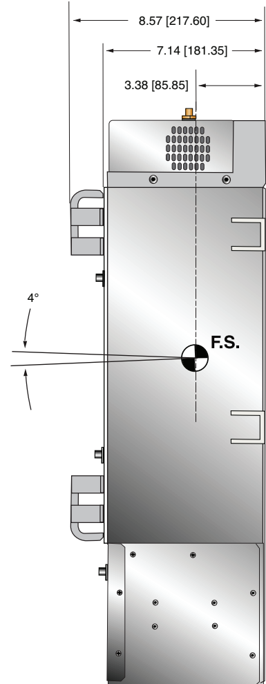
SIDE VIEW
