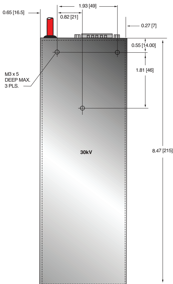
BOTTOM VIEW
