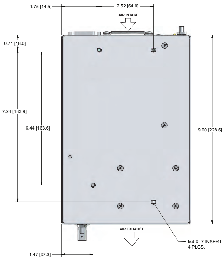
BOTTOM VIEW
