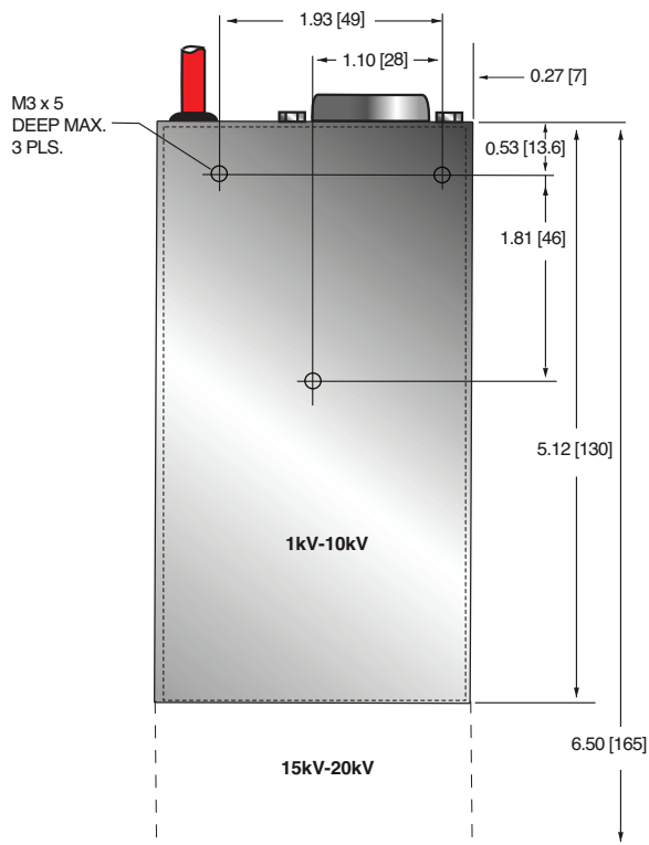
BOTTOM VIEW
