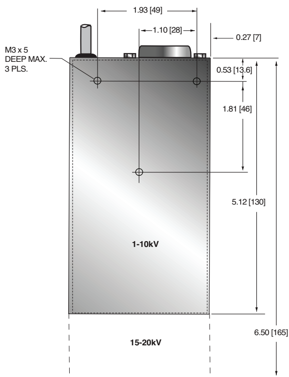
BOTTOM VIEW
